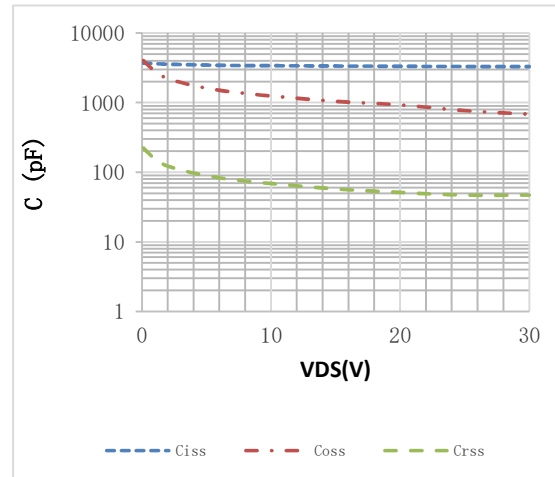
Fig.2 Capacitance Characteristics
